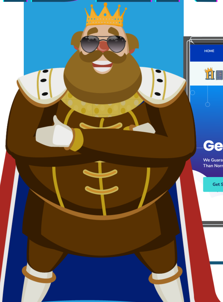
MASCOT
